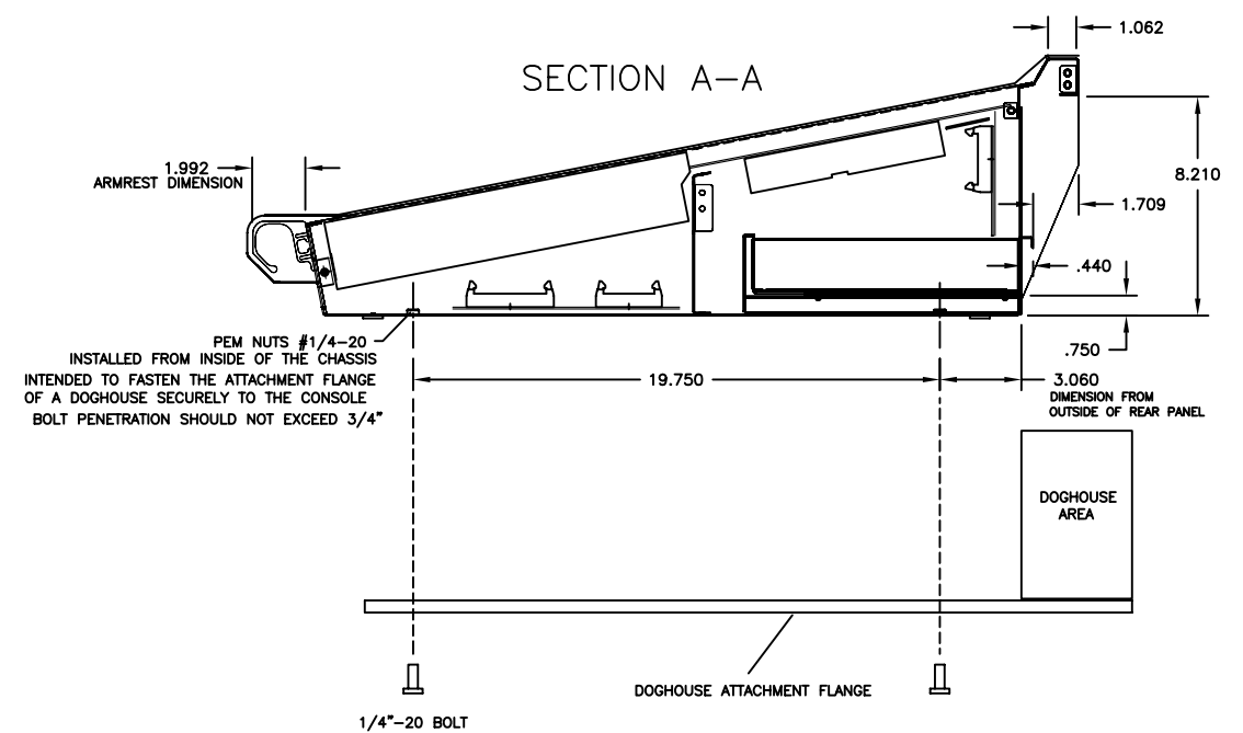
VARIABLE LENGTH PER CHASSIS SIZE
